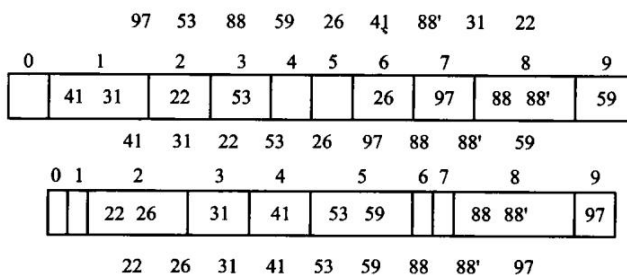
(b) 低位优先
