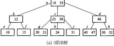
(a) 3阶B树
