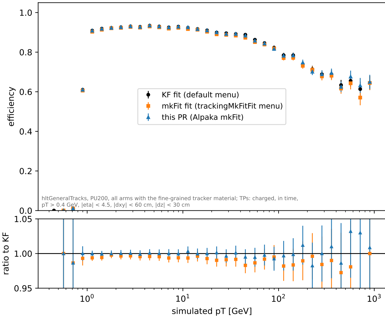
qcd: efficiency vs simulated pT
