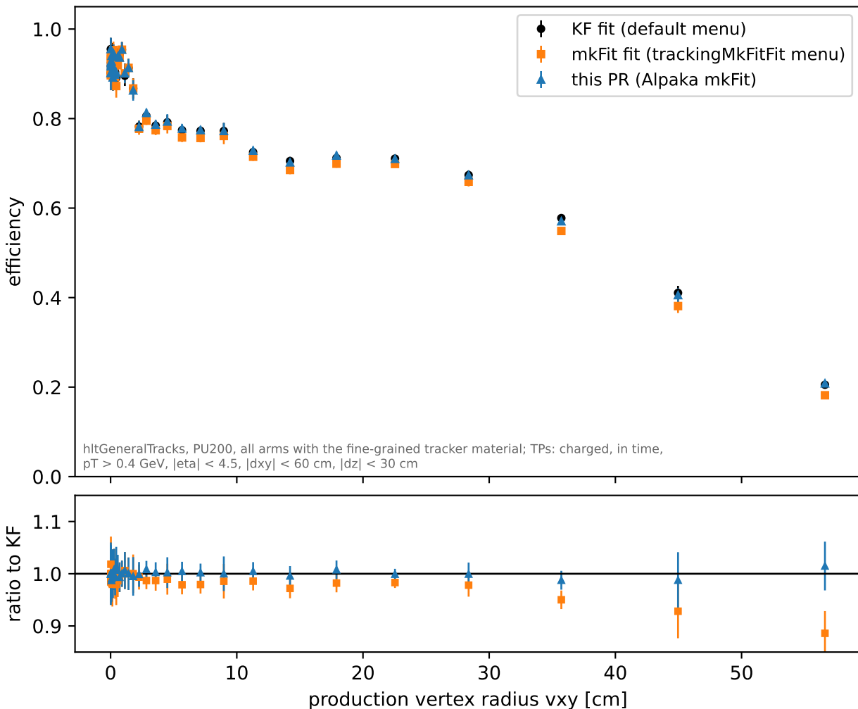
qcd: efficiency vs production vertex radius vxxy
