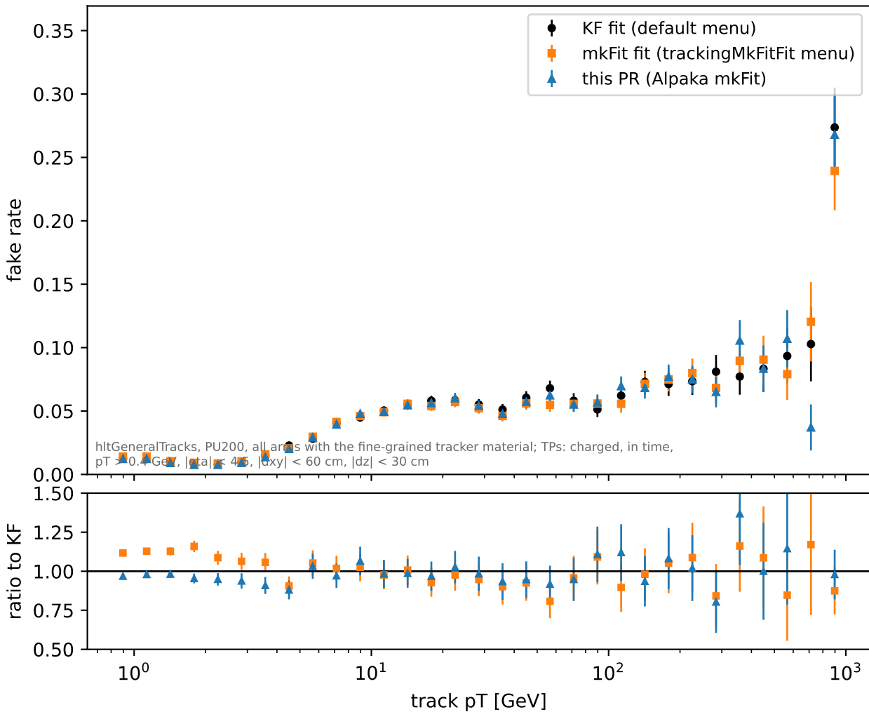
qcd: fake rate vs track pT
