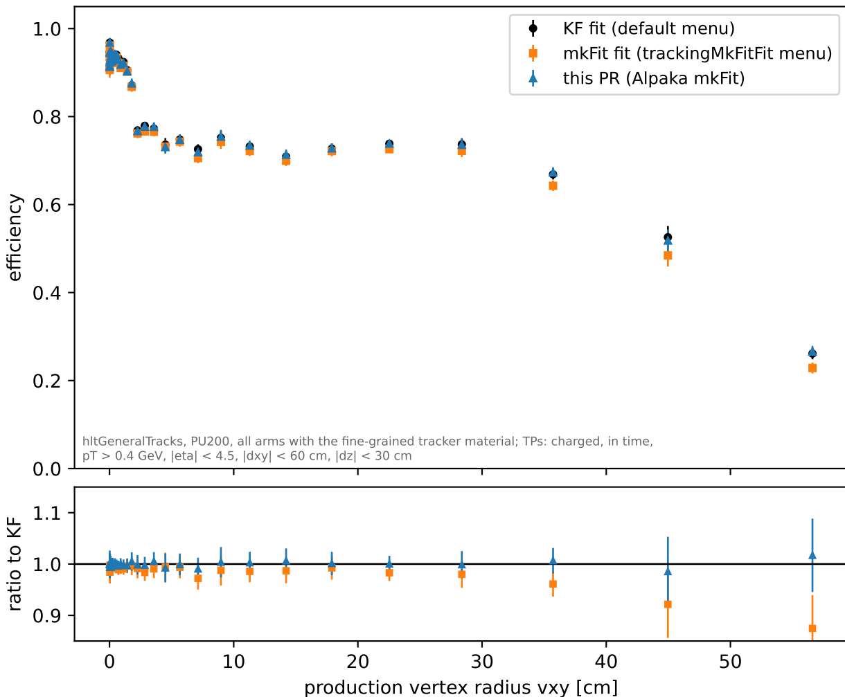
ttbar: efficiency vs production vertex vx
