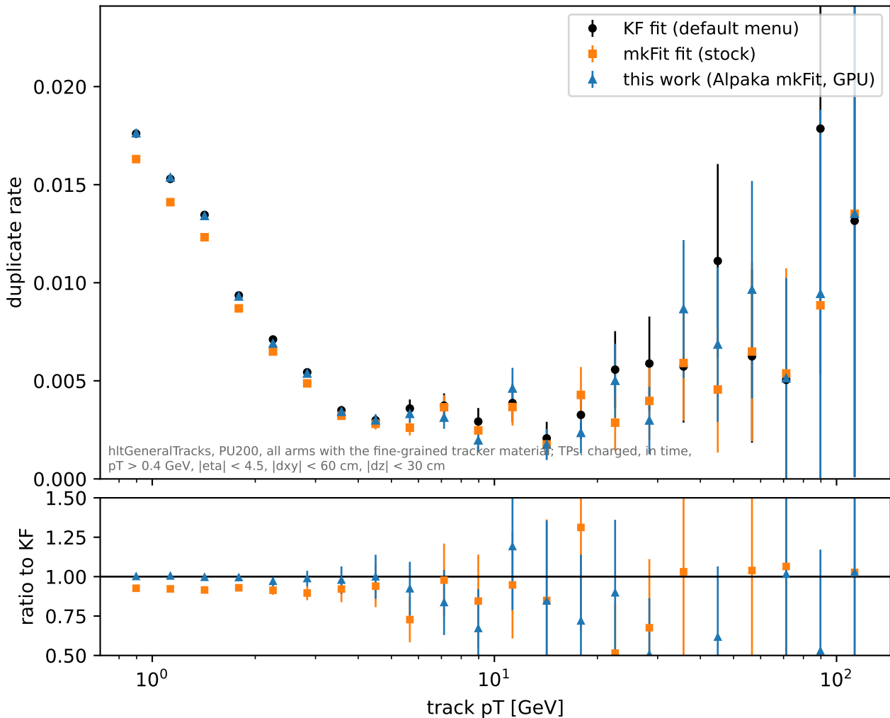
t\bar{t} : duplicate rate vs track p_T
