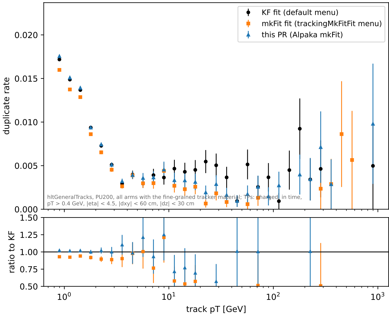
qcd: duplicate rate vs track pT
