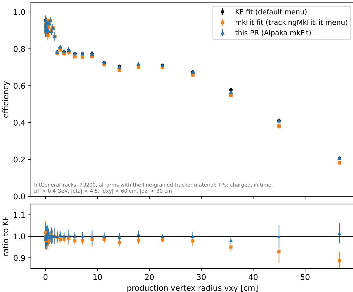
qcd: efficiency vs production vertex radius v_{xy}
