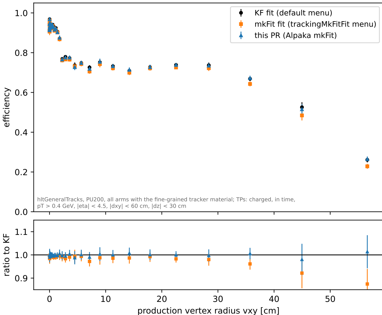
ttbar: efficiency vs production vertex radius vxxy
