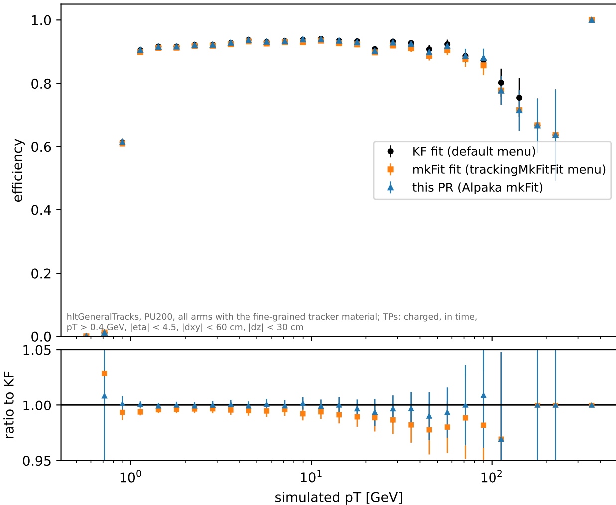
ttbar: efficiency vs simulated pT
