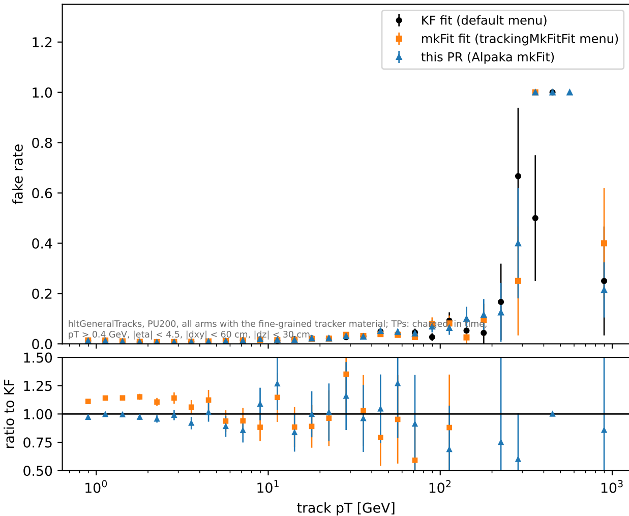
ttbar: fake rate vs track pT
