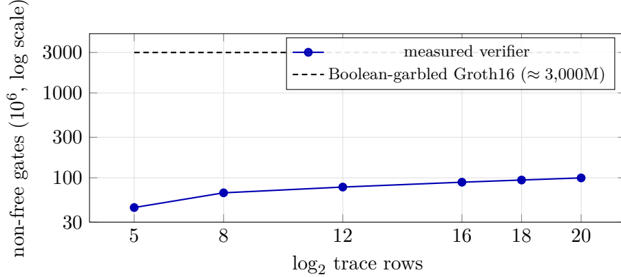
Figure 3: On a logarithmic vertical axis, the measured verifier grows from 44.6M non-free gates at 2^5 rows to 99.6M at 2^{20} , a 2.2\times increase for a 32,768\times larger trace. The dashed line shows the approximately 3,000M-gate Boolean-garbled Groth16 comparator.
