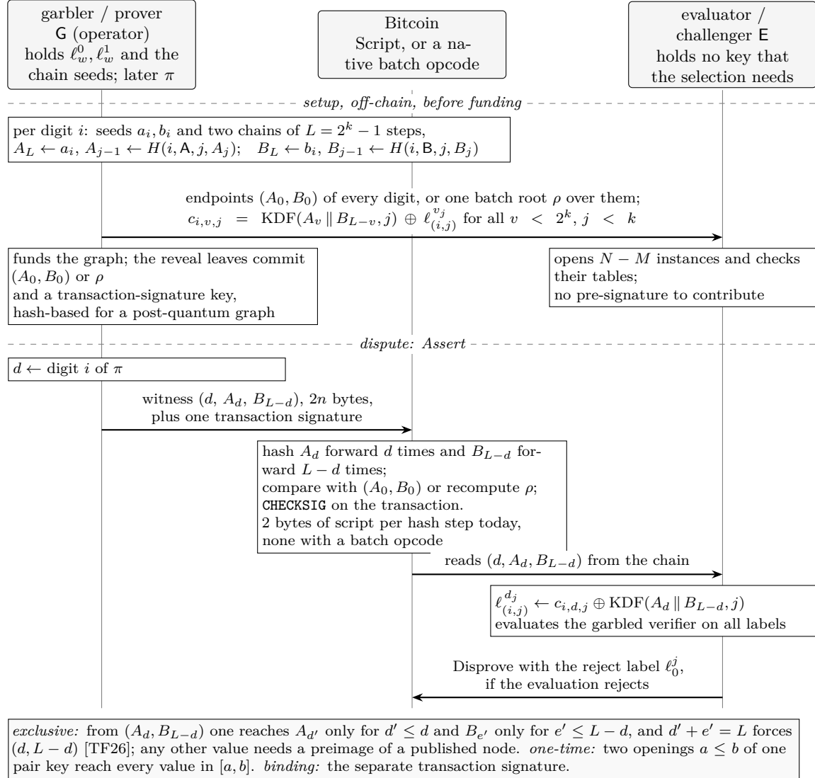
Figure 4: Hash-based label selection for one k -bit digit position i with n -byte chain nodes. The selection material is two nodes instead of one signature, the evaluator contributes nothing at setup, and the transaction binding that the adaptor gets from the same signature must be added separately. Verification is a hash ladder, in Script today or in a batch opcode under the soft fork of Table 5.
