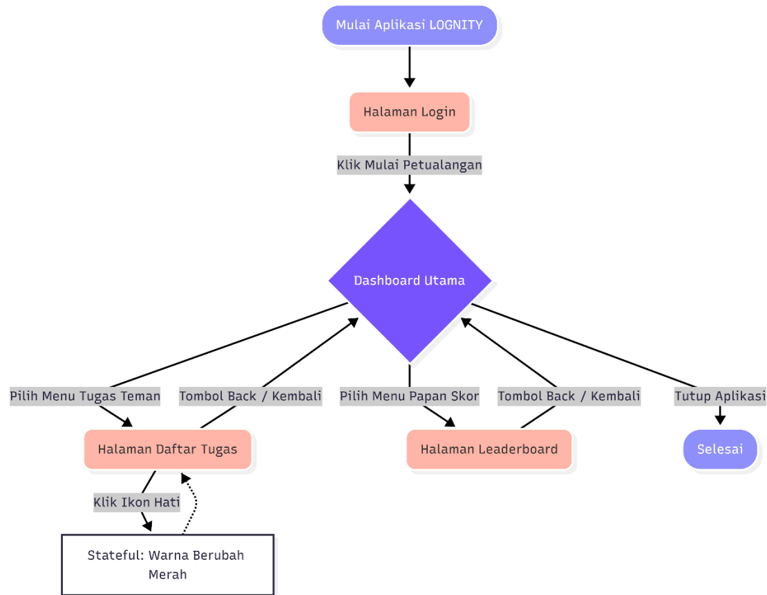
Gambar 1. Flowchart Lognity Mobile
