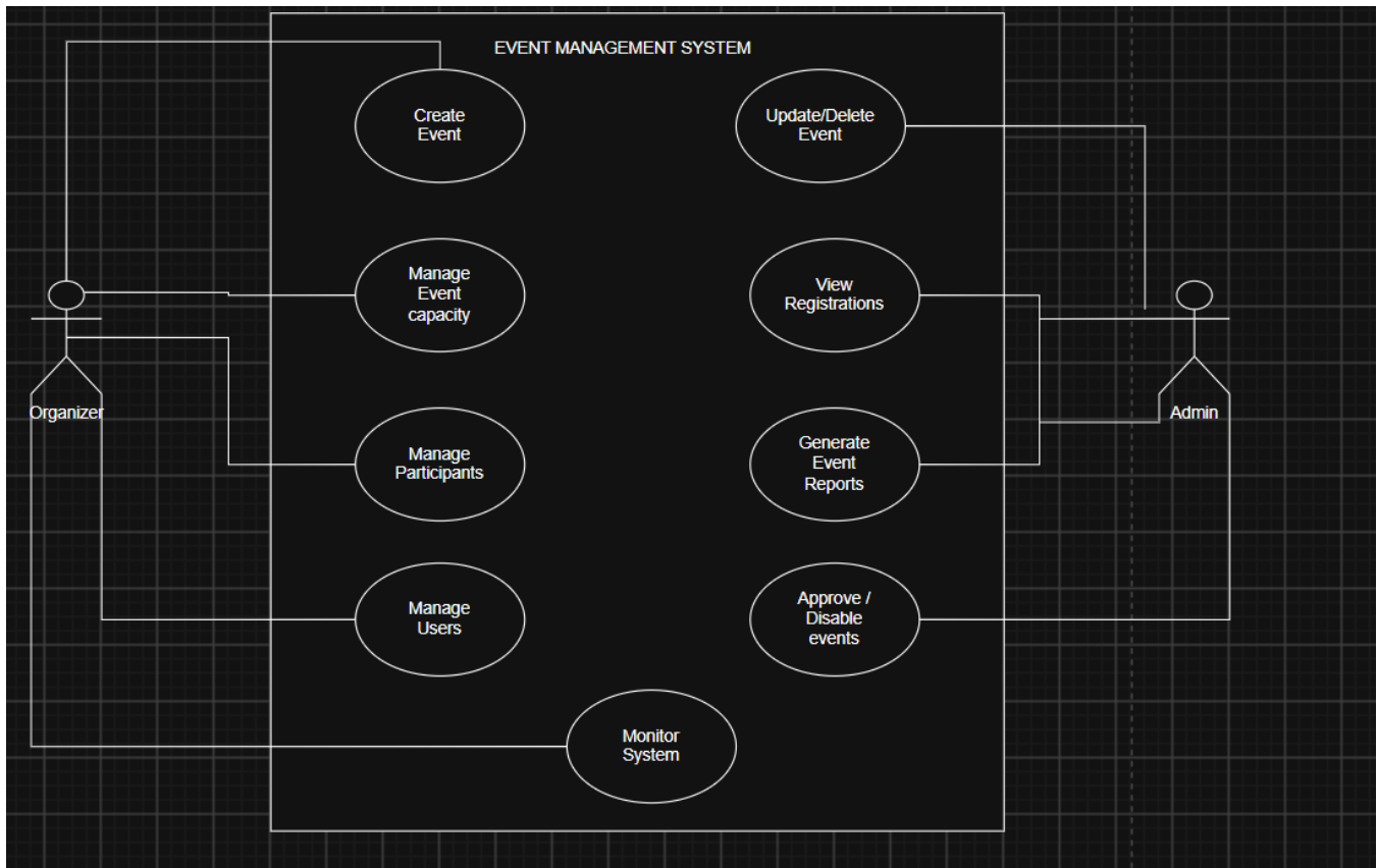
Use-case diagram 2: Organizer and Administrator interactions with the Event Management System.
