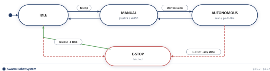
Figure 3.13 – Robot operating-mode state diagram
