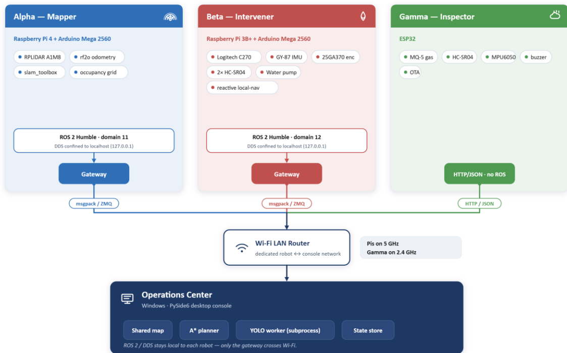
Figure 3.4 – Overall multi-robot system architecture
