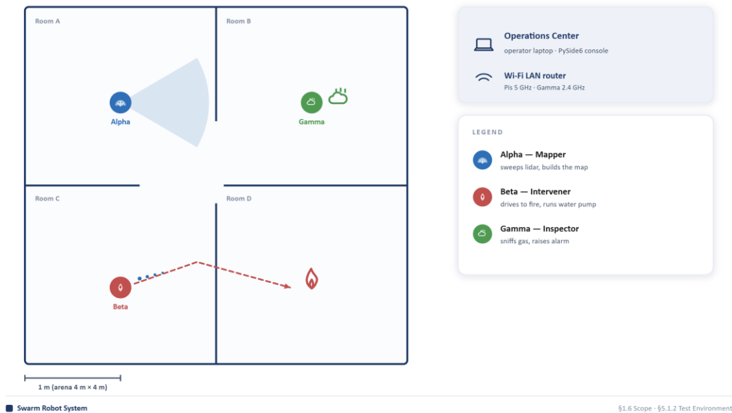
Figure 5.1 – Indoor test deployment scenario
