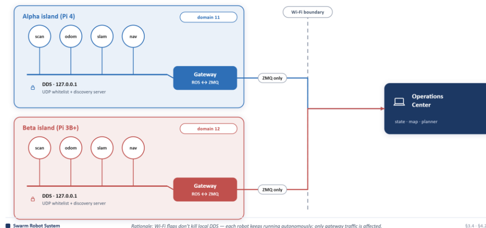
Figure 3.5 – ROS-island isolation and the gateway boundary
