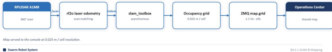
Figure 4.2 – SLAM and mapping pipeline
