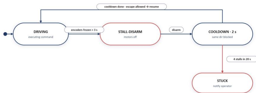
Figure 4.5 – Stall-detection and anti-lockup state machine
