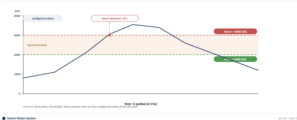
Figure 5.5 – Gas-alarm threshold and hysteresis behaviour
