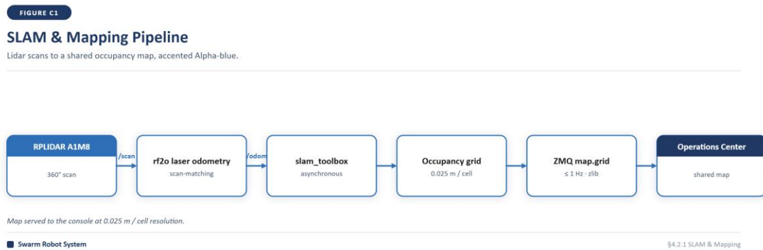
Figure 4.2 – SLAM and mapping pipeline
