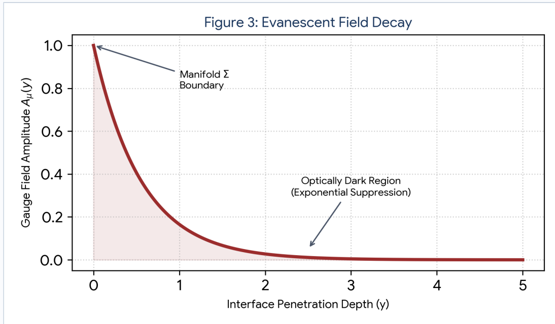
Figure 3: Evanescent Field Decay. A mathematical plot showing the amplitude of a gauge field A_\mu(y) decaying exponentially as it penetrates the interface \Sigma . Demonstrates why the twin manifold remains optically dark.
