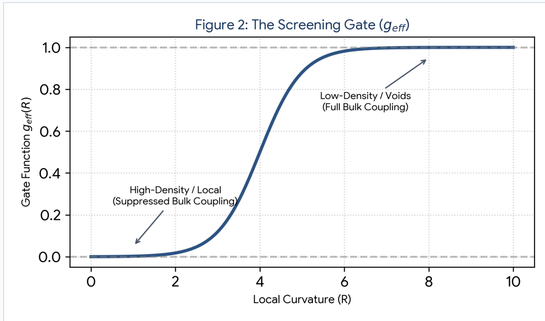
Figure 2: The Screening Gate ( g_{eff} ). A plot of the gate function g_{eff}(R) vs. local curvature ( R ). Shows the sharp transition from 0 (high-density/local) to 1 (low-density/voids), representing the suppression of bulk coupling in local gravity environments.
