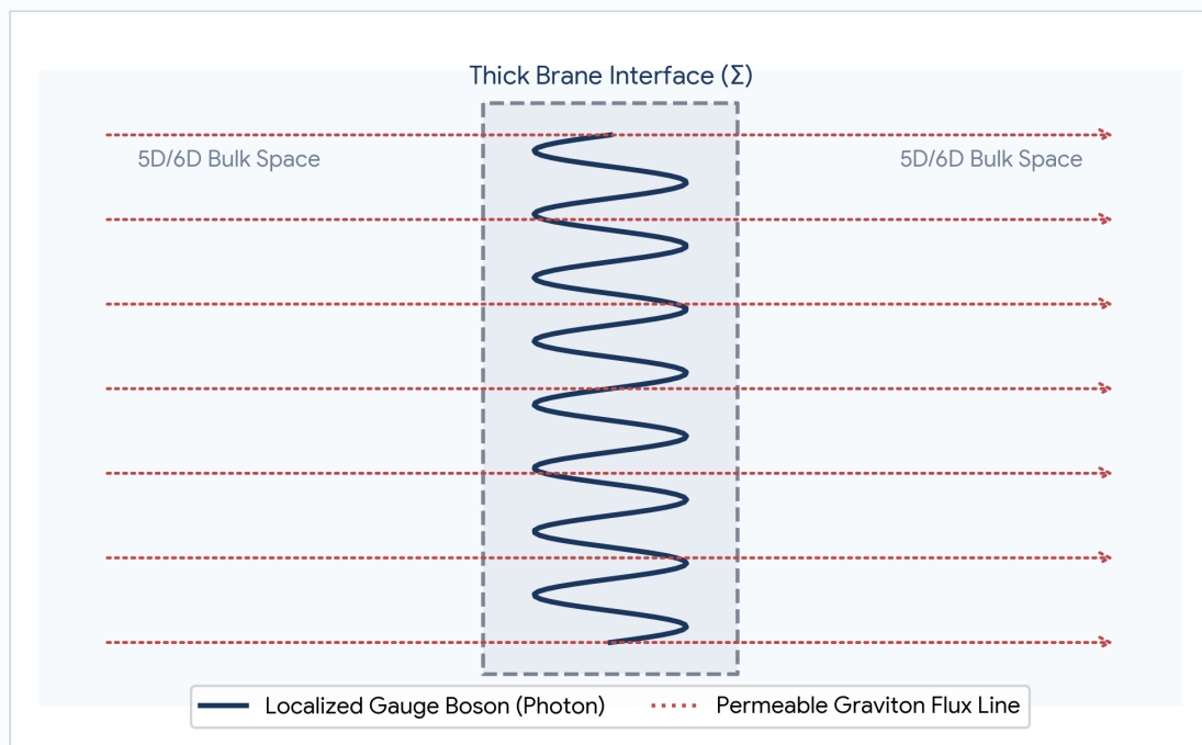
Figure 1: The Thick Brane Interface ( \Sigma ). A cross-sectional view of our 4D manifold showing finite topological 'thickness' within the 5th and 6th dimensions, illustrating gauge boson (photon) localization vs. graviton permeability.
