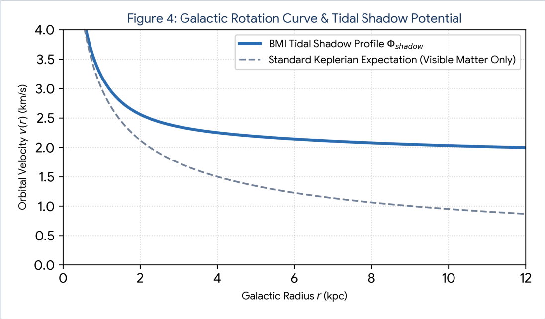
Figure 4: Tidal Shadow Potential (Dark Matter). A conceptual diagram showing the 'shadow' potential \Phi_{shadow} projected by the twin manifold's mass distribution, showing how it flattens rotation curves without requiring dark matter haloes.
