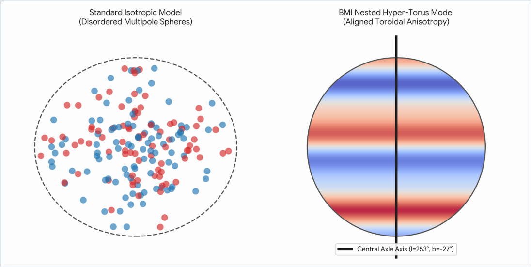
Figure 5: Axis of Evil Anisotropy. A projection of the CMB showing the low-multipole moments ( l=2, l=3 ) aligned along a preferred vector n_i , derived from the orientation of the hyperspatial shear tensor S_{\mu,\nu} .
