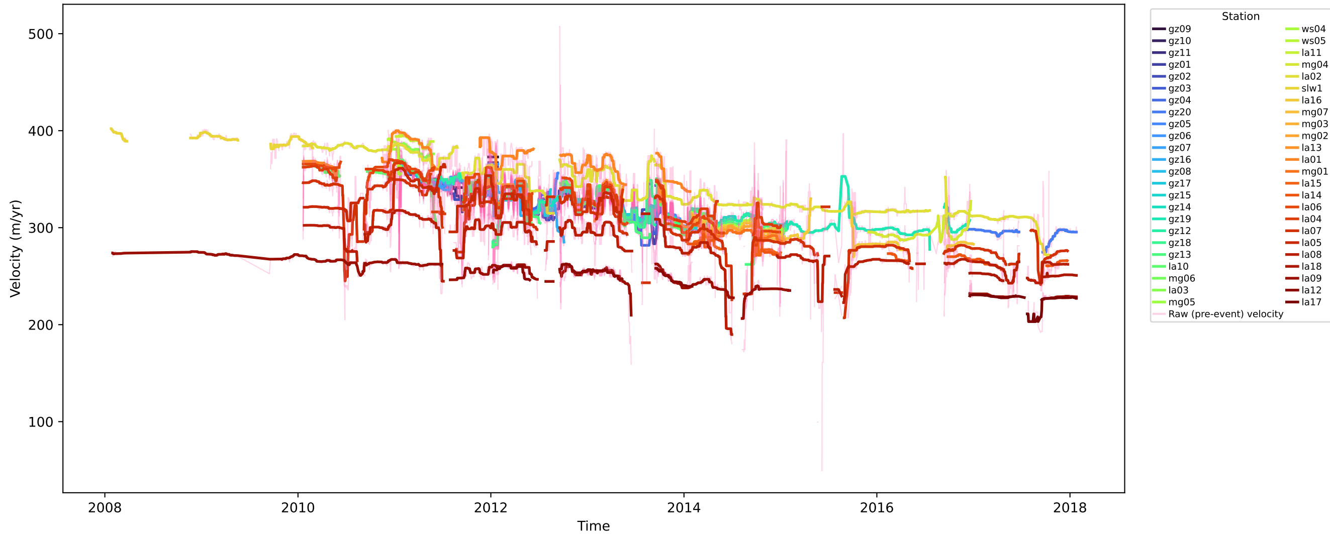
Figure 4: Velocity Time Series by Station
