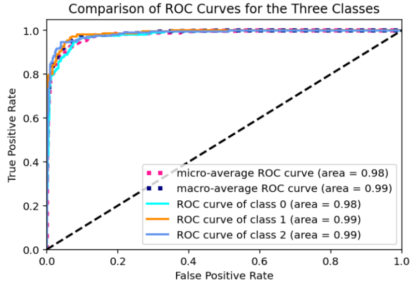
Figure 0.2: Figure 2. Receiver operating characteristic comparison for the three classes using test data from subject 16. Source: Wickramaratne and Mahmud [1].
