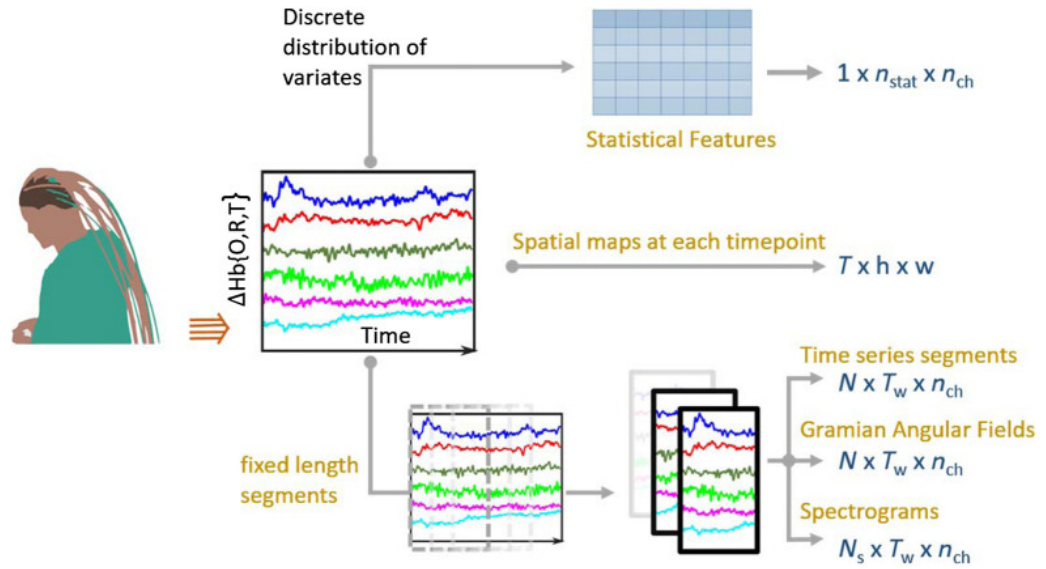
Figure 0.5: Figure 5. Extraction of samples for training neural networks from fNIRS data. Source: Eastmond et al. [6].
