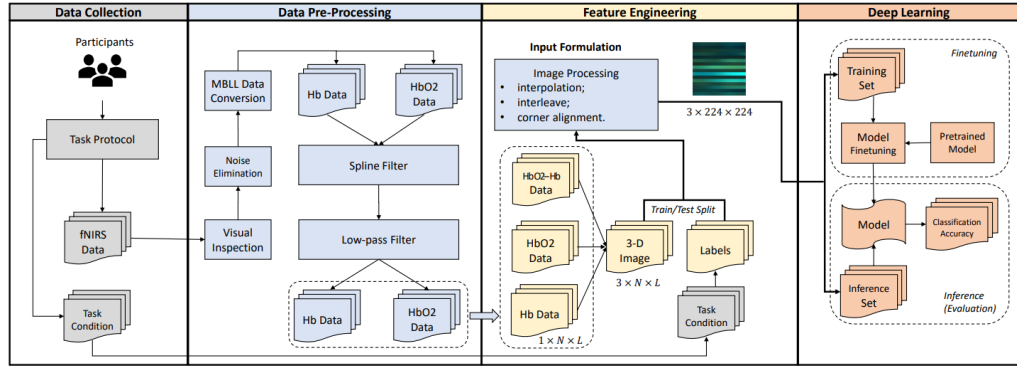
Figure 0.6: Figure 6. Proposed framework for walking-task classification using fNIRS data. Source: Ma et al. [7].
