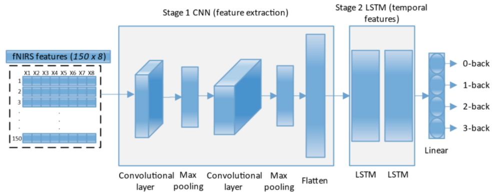
Figure 0.3: Figure 3. Proposed architecture incorporating CNN and LSTM layers for fNIRS workload classification. Source: Khan et al. [5].
