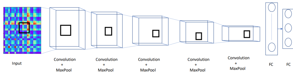
Figure 0.1: Figure 1. The proposed convolutional neural network used for fNIRS task classification. Source: Wickramaratne and Mahmud [1].
