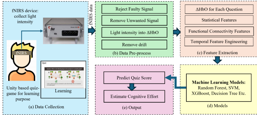
Figure 0.9: Figure 9. Overview of the machine-learning pipeline for estimating cognitive effort from fNIRS data. Source: Sharmin et al. [8].
