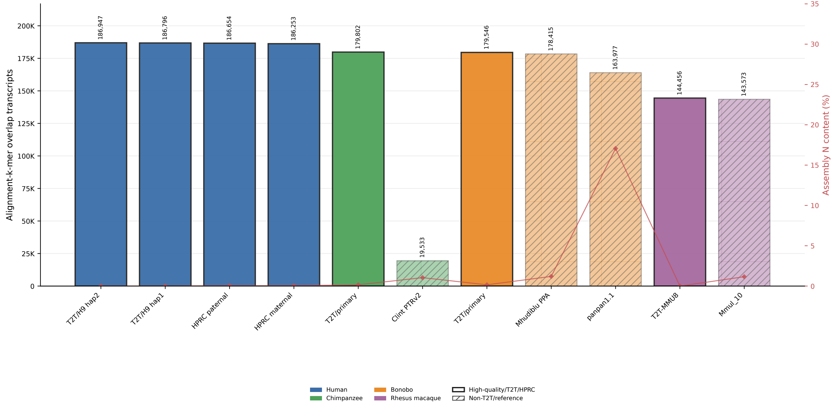
Assembly-wise high-confidence alignment and k-mer overlap (k=24)
