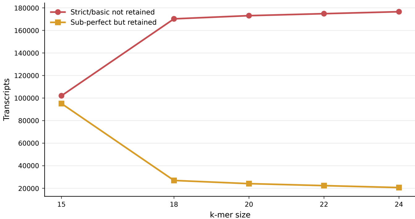
Rare non-perfect k-mer outcomes by k
