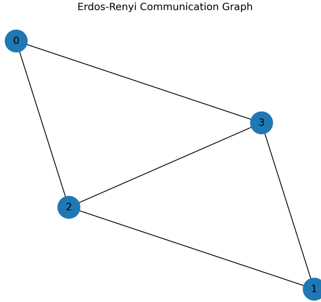
Figure 4: Connected Erdős–Rényi communication graph.
