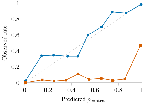
Figure 4: Reliability of p_{\text{contra}} on the SICK test half, ten bins. The dashed diagonal is perfect calibration, where a predicted probability equals the observed rate. The fine-tuned head tracks it, the off-the-shelf head falls far below.
