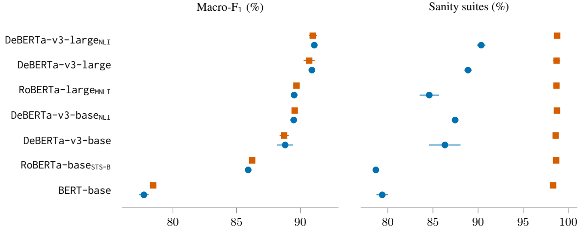
Figure 2: Macro-F 1 (left) and sanity-suite accuracy (right) per encoder. RAW and AUG : mean over ten random seeds, bars one standard deviation.
