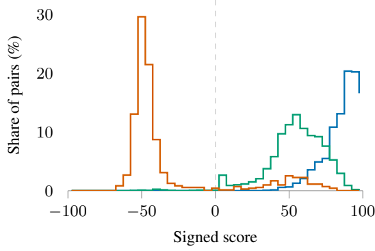
Figure 3: Signed score by gold class (Equation 1, one polarity head), bins of width 5: entailment , neutral , contradiction . Dashed line: zero.
