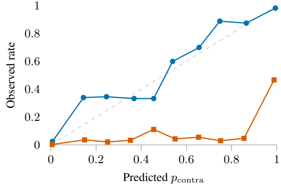
Figure 4: Observed contradiction rate against predicted p_{\text{contra}} , SICK test half, ten bins, for the fine-tuned head and the off-the-shelf head . Dashed diagonal: perfect calibration.
