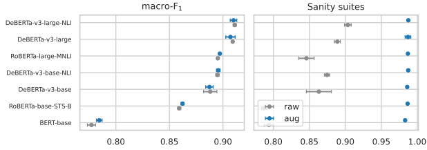
Figure 1: Augmentation moves one axis and not the other. Points are means over ten seeds, bars one standard deviation. The task axis is unchanged within noise; the sanity axis converges to a single value from seven different starting points.
