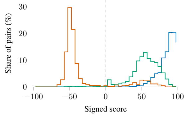
Figure 3: Signed score by gold class on the SICK test half at \alpha = 2 , bins of width 5: entailment ( n = 1404 ), neutral ( n = 2000 ), contradiction ( n = 712 ). The dashed vertical line marks zero, where the sign changes.
