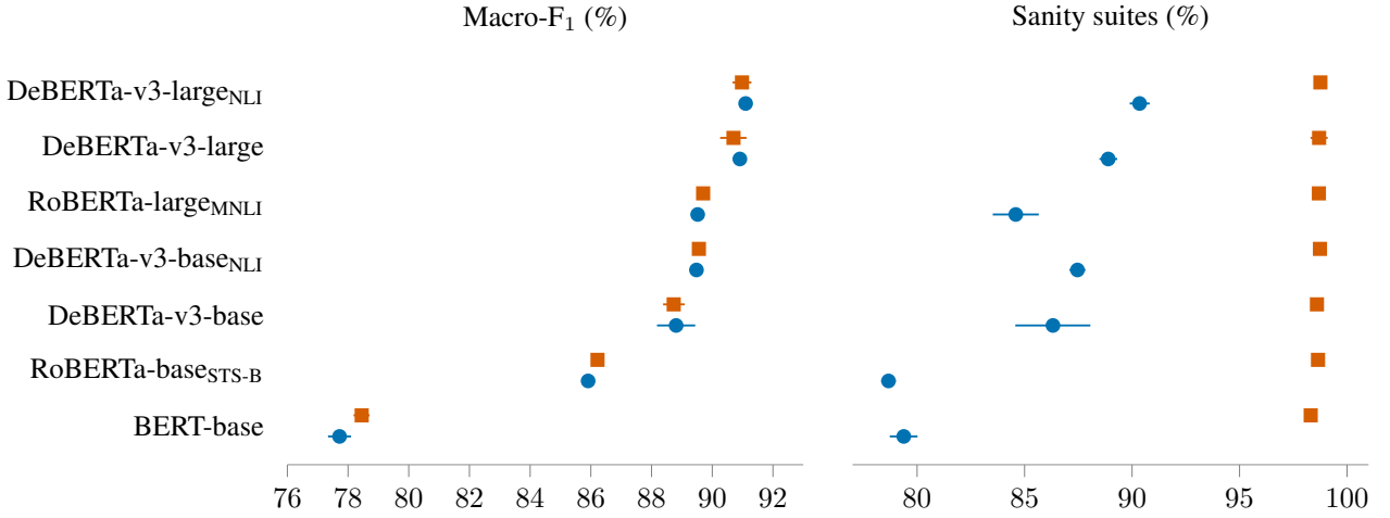
Figure 2: Augmentation moves one axis and not the other. RAW and AUG : means over ten seeds, bars one standard deviation. The panels do not share an x range.
