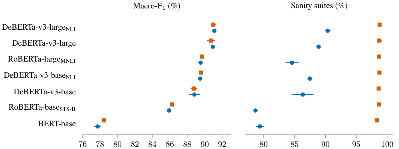
Figure 2: Augmentation moves one axis and not the other. RAW and AUG : means over ten seeds, bars one standard deviation. The panels share no x range.
