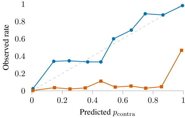
Figure 4: Reliability of p_{\text{contra}} , SICK test half, ten bins. The dashed diagonal is perfect calibration. The fine-tuned head tracks it, the off-the-shelf head falls far below.
