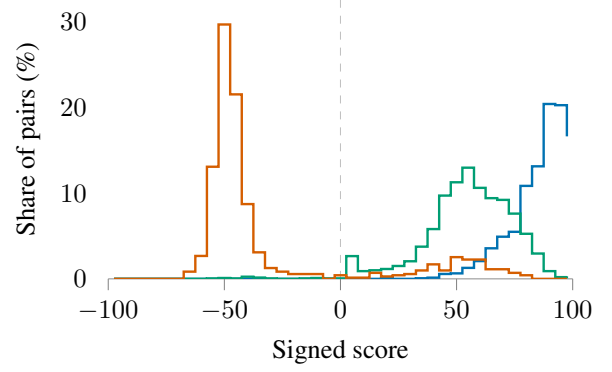
Figure 3: Signed score by gold class, SICK test half at \alpha = 2 , bins of width 5: entailment ( n = 1404 ), neutral ( n = 2000 ), contradiction ( n = 712 ). Dashed line: zero.
