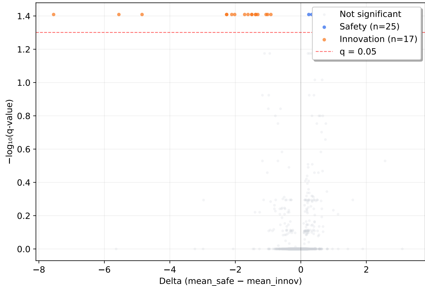
Volcano Plot: Feature Polarization with FDR Correction
