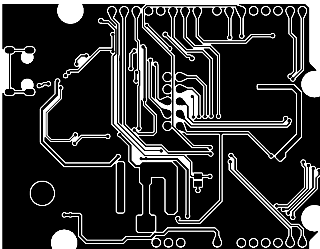
Bottom Copper
