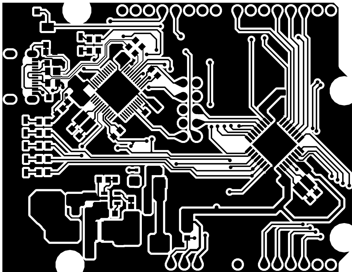
Top Copper
