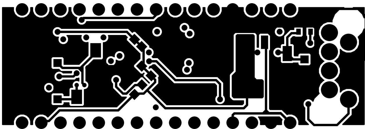
Bottom Copper
