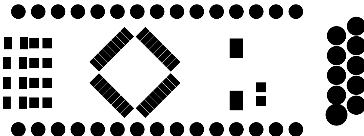
Soldermask Top
