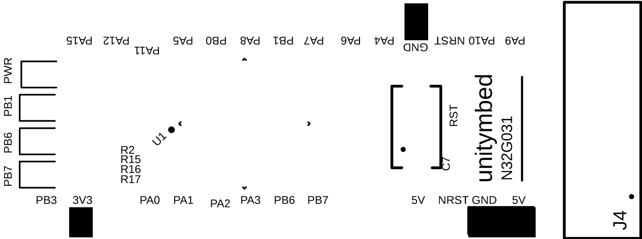
Silkscreen Top
