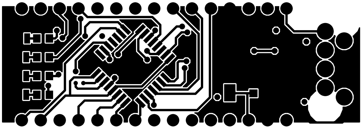
Top Copper
