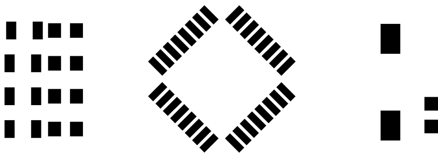
Solderpaste Top
