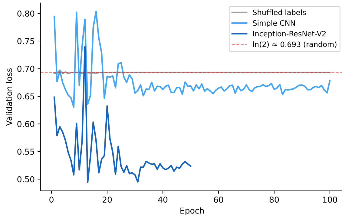
Validation loss over training
