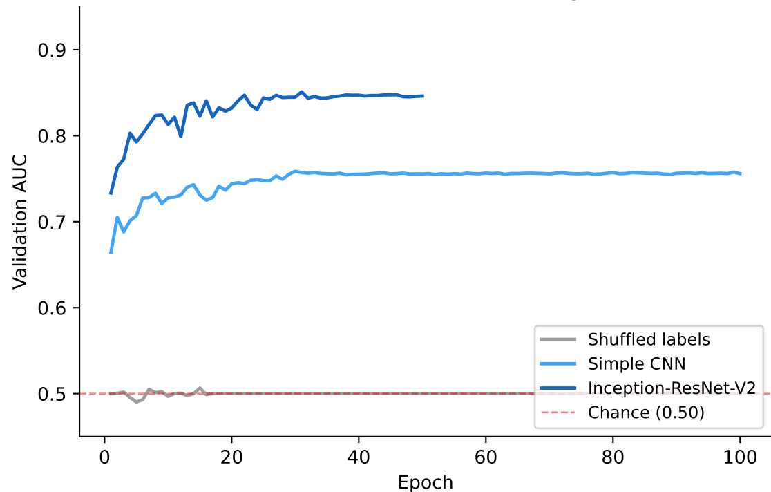
Validation AUC over training
