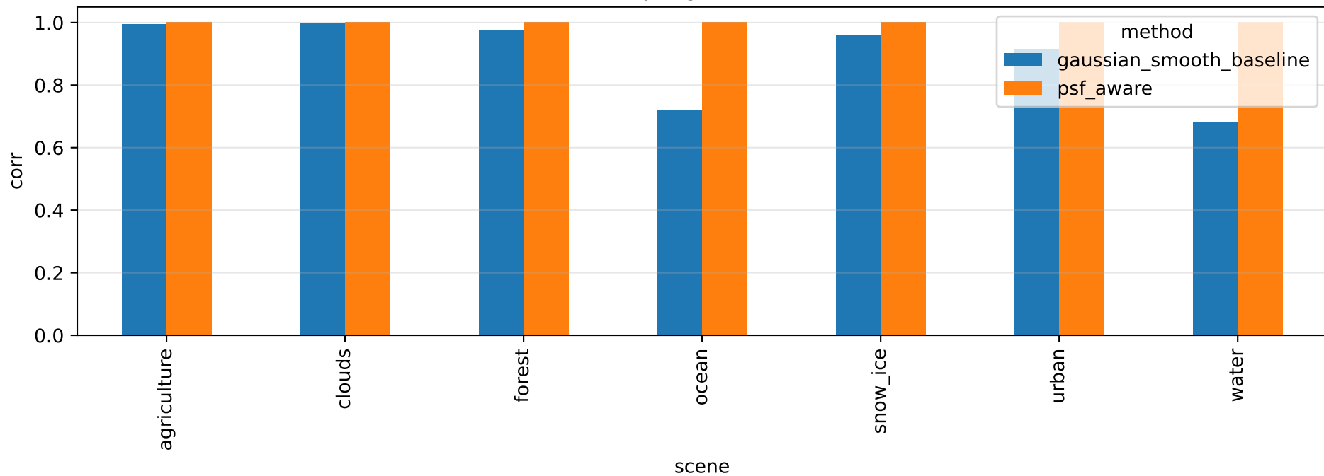
Resampling metric: corr
