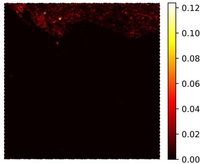
Bilinear forest RMSE=3.11e-03
