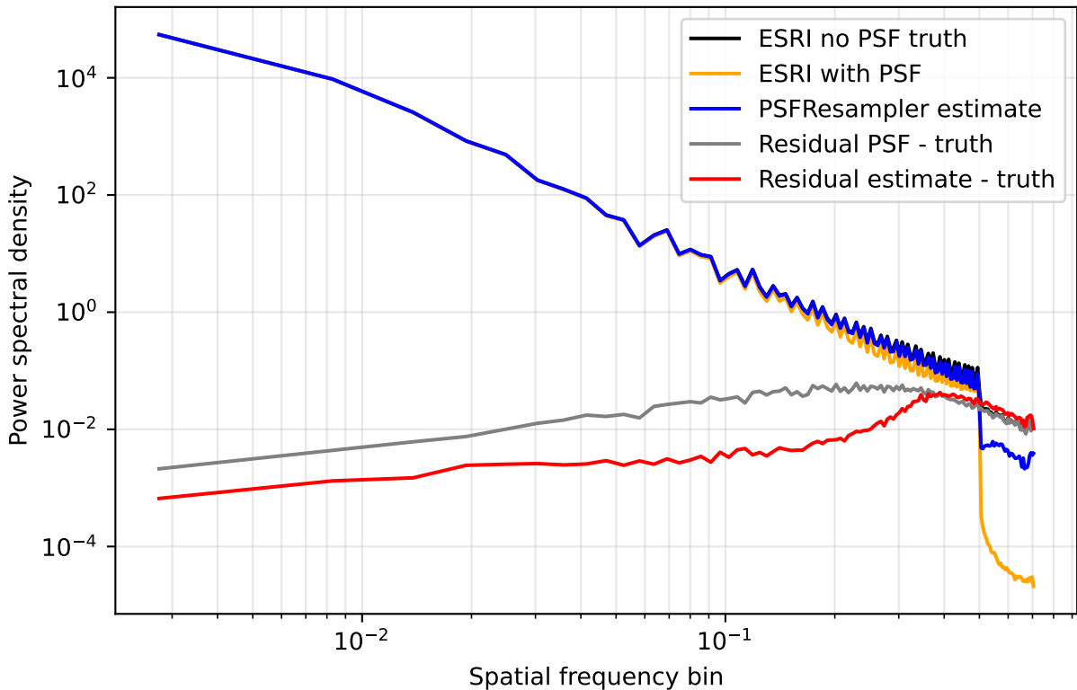
Synthetic detector HEALPix PSD: forest
