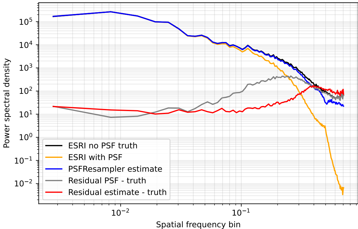
Synthetic detector HEALPix PSD: urban
