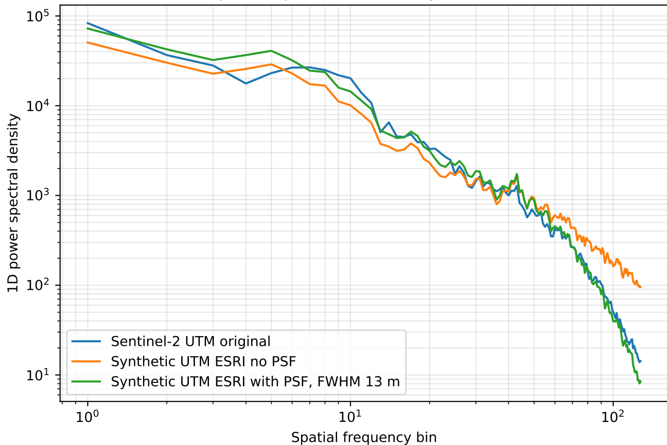
UTM power spectra consistency check: urban
