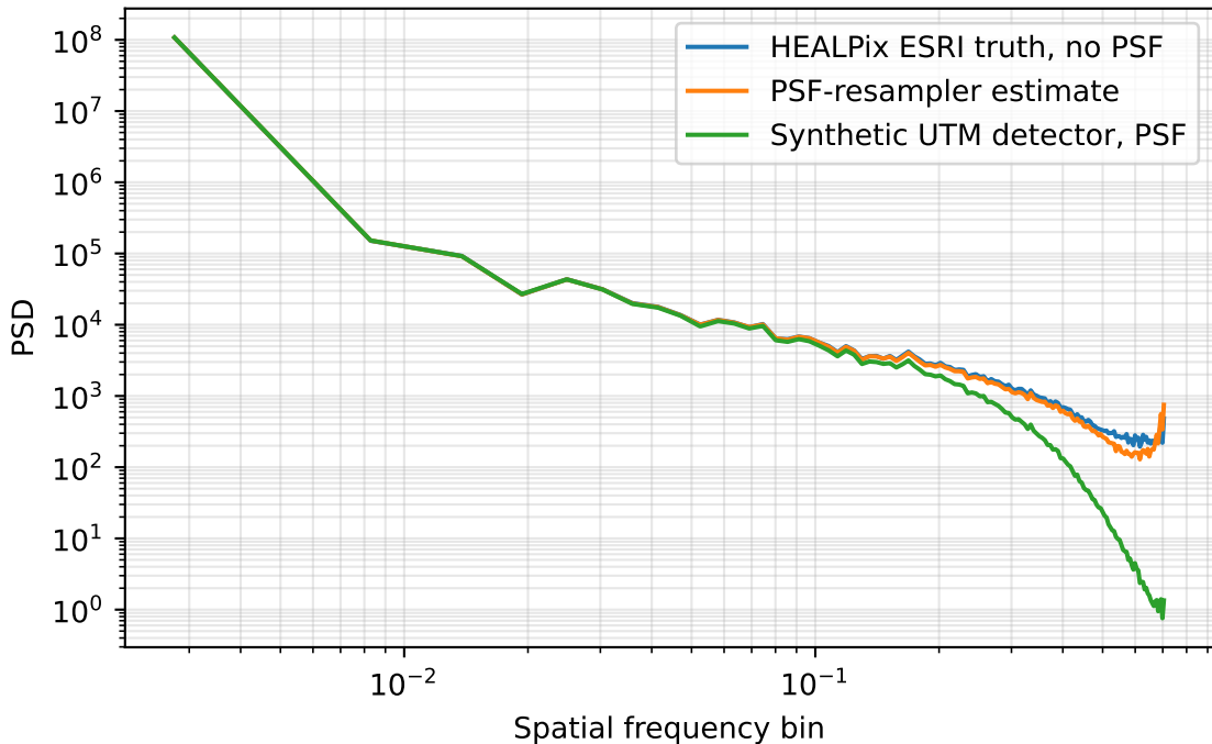
Synthetic detector PSD: urban
