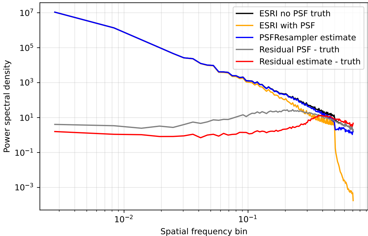
Synthetic detector HEALPix PSD: agriculture
