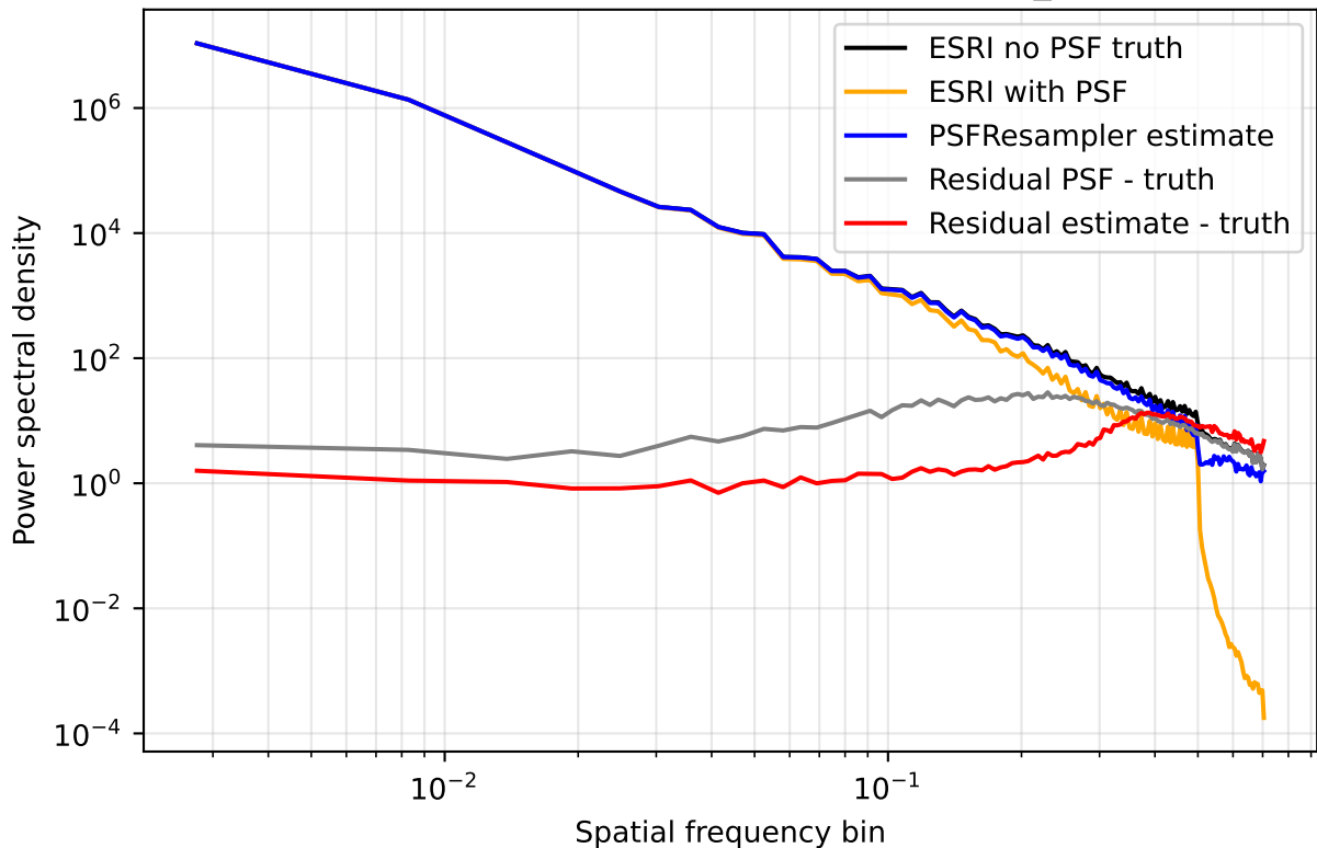
Synthetic detector HEALPix PSD: snow_ice
