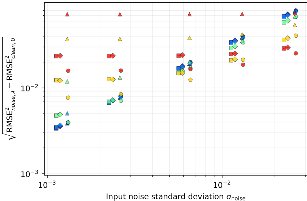
White noise
