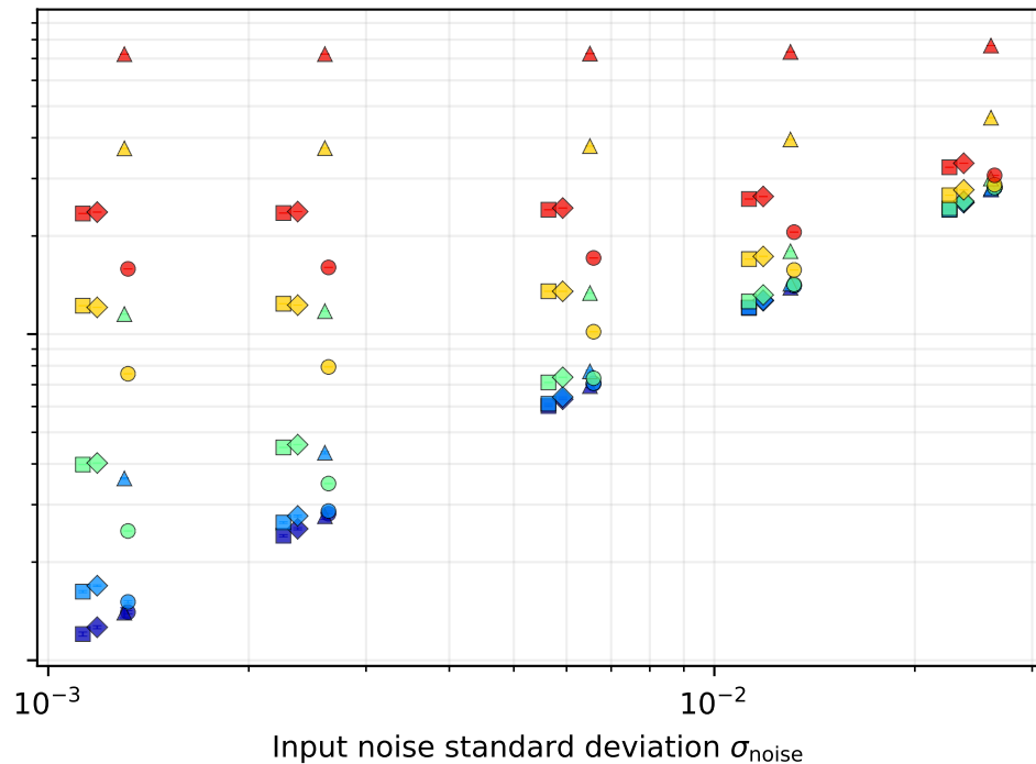
Correlated noise
