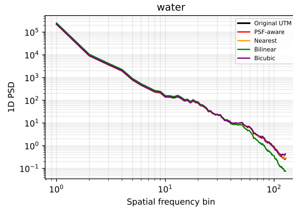
Round-trip 1D power spectra — original vs reconstructed (all methods)
