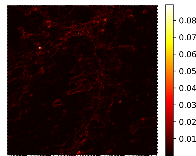
Bicubic agriculture RMSE=2.92e-03
