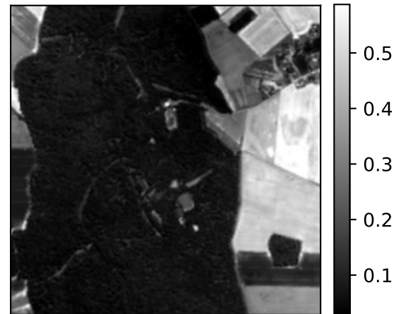
PSFResampler estimate
