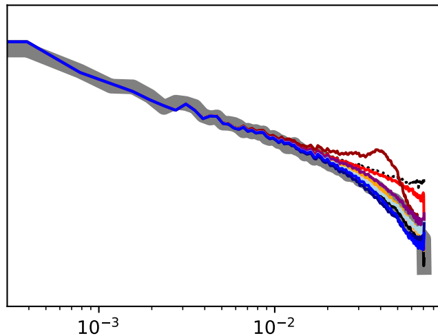
Forest
