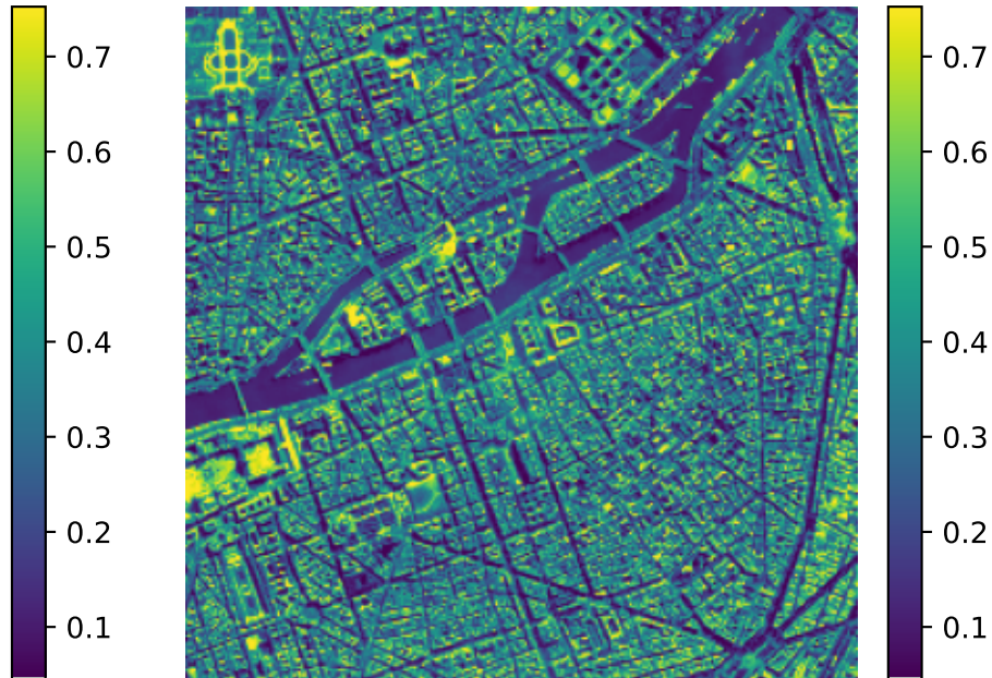
Inverse-only check: exact HEALPix values \rightarrow UTM reconstruction HEALPix \rightarrow UTM only (method=cubic, exact cell values in)
