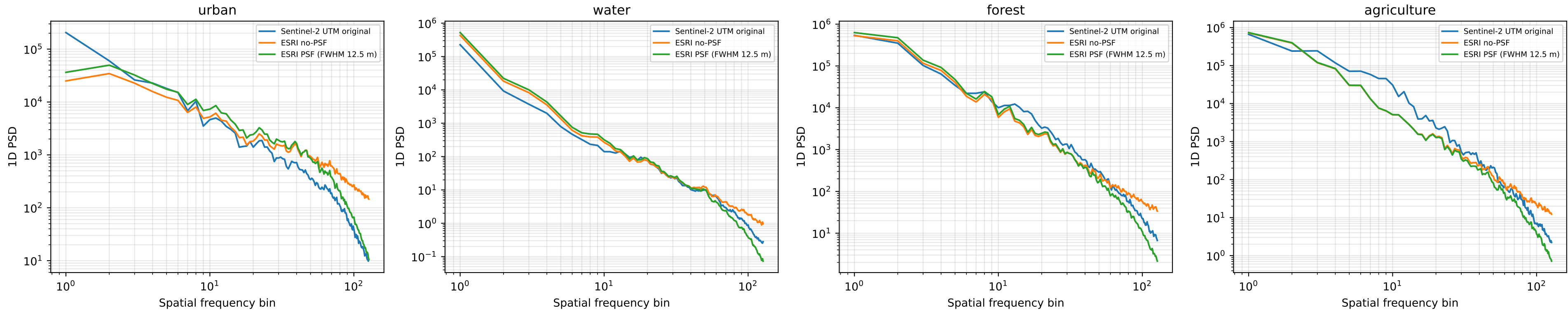
urban — Sentinel-2
