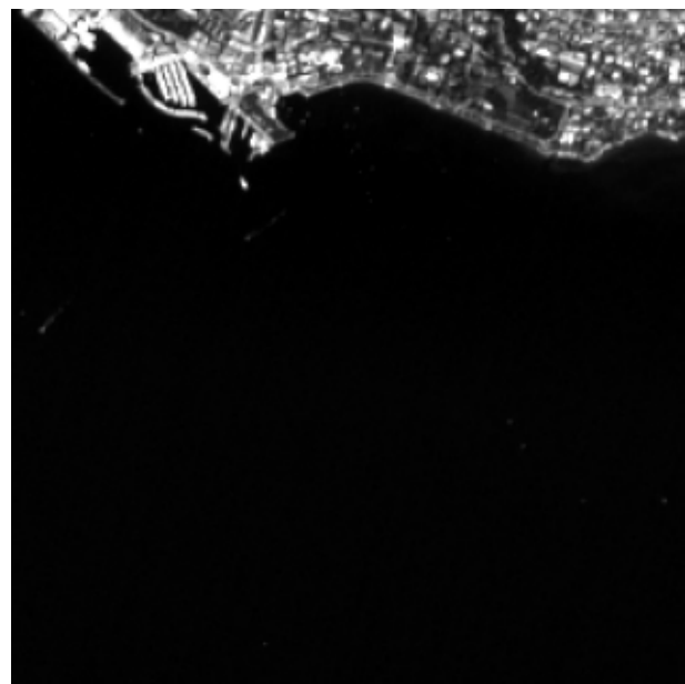
water — Sentinel-2
