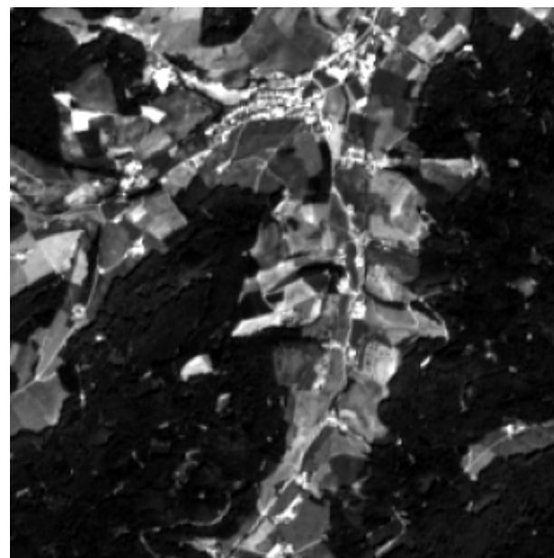
forest — Sentinel-2
