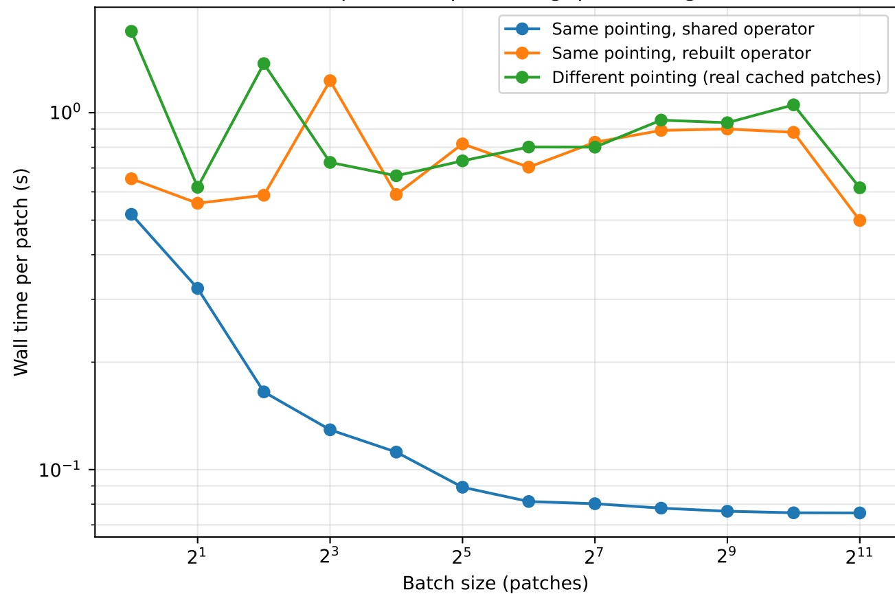
healpix-resample throughput scaling
