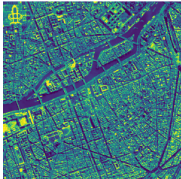
urban True UTM (no-PSF)
