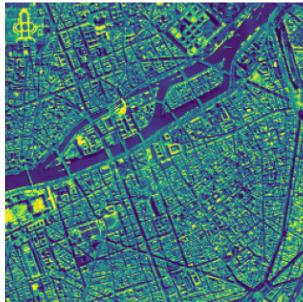
HEALPix \rightarrow UTM only (method=cubic, exact cell values in)
